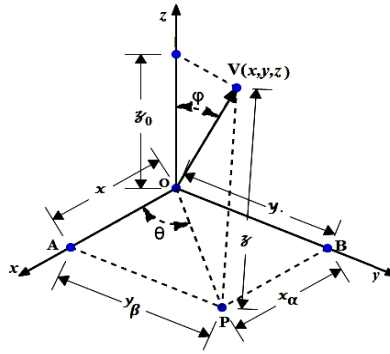
Fig. 8 Reference voltage vector calculation
