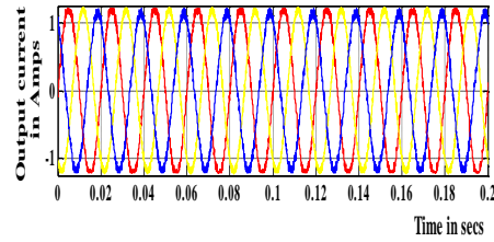
Fig. 12 Three phase current waveform
