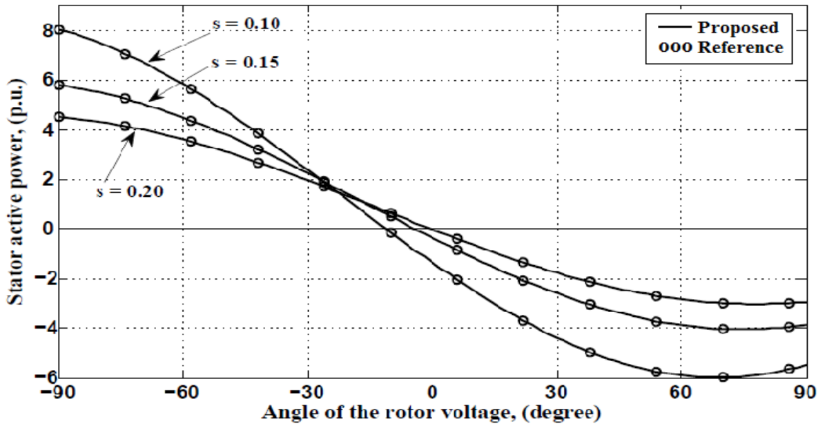
Fig. 3 Stator active power versus the angle of the rotor voltage
