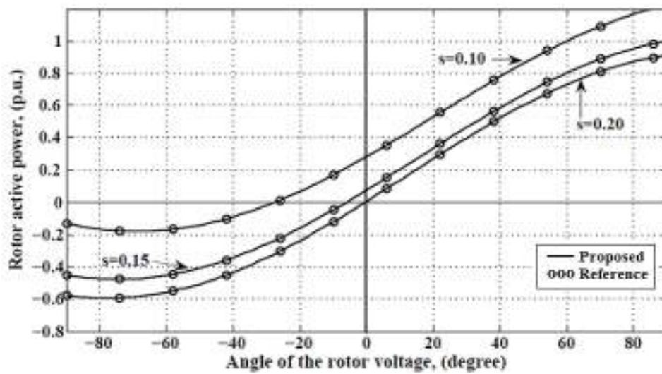
Fig. 5 Rotor active power versus the angle of the rotor voltage
