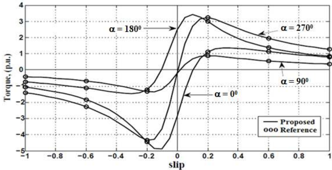
Fig. 12 Electromagnetic torque versus the slip
