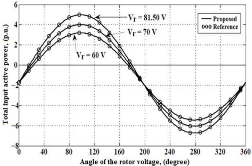
Fig. 11 Total input active power versus the angle of the rotor voltage
