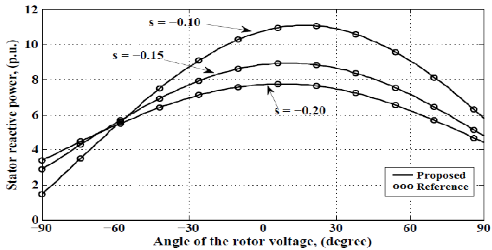
Fig. 7 Stator reactive power versus rotor voltage phase angle
