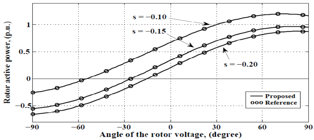
Fig. 8 Rotor active power versus rotor voltage phase angle
