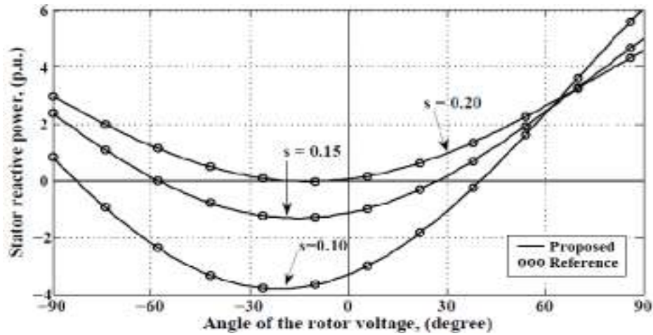
Fig. 4 Stator reactive power versus the angle of the rotor voltage
