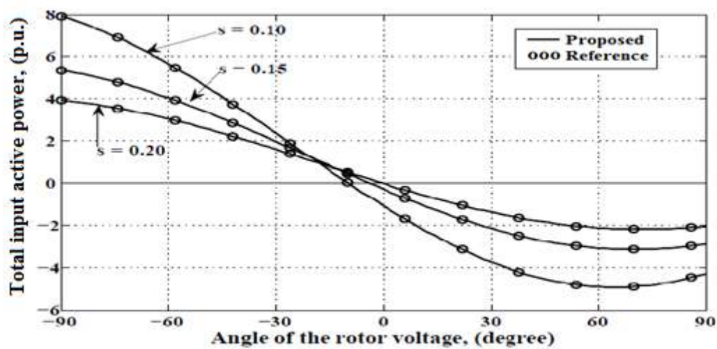
Fig. 9 Total input active power versus the angle of the rotor voltage
