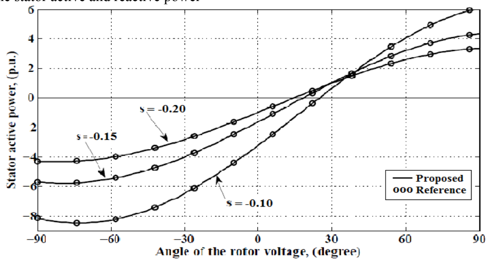
Fig. 6 Stator active power versus the angle of the rotor voltage
