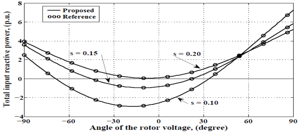
Fig. 10 Total input reactive power versus the angle of the rotor voltage
