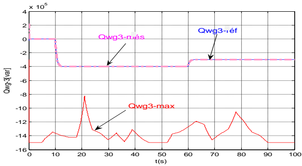
(d) reactive power produced by the third wind generator
