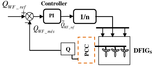
(b) Reactive power control
