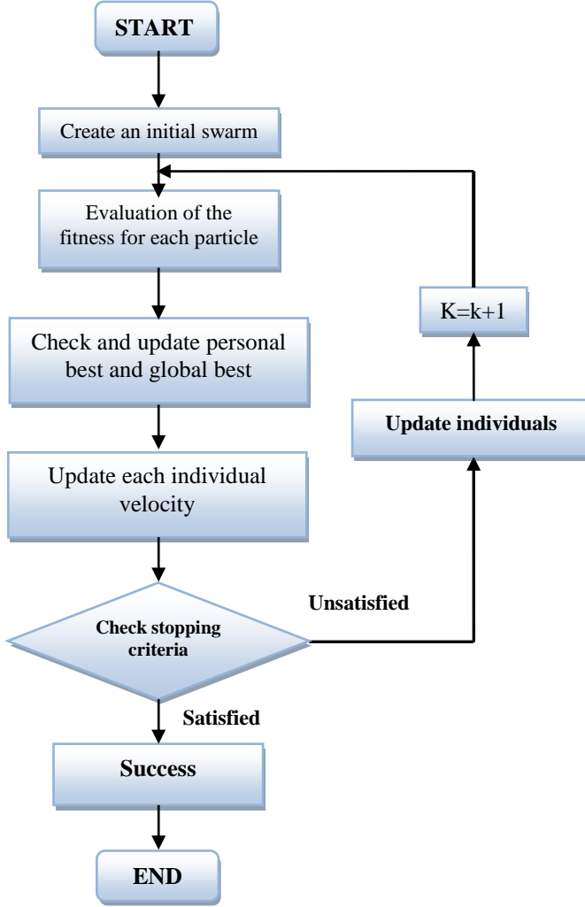
Figure 4. Flowchart of the PSO procedure [26]
