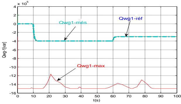
(b) reactive produced by the first wind generator
