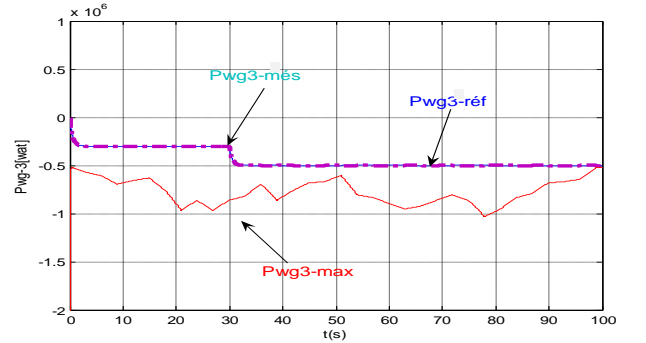
(d) active power produced by the third wind generator
