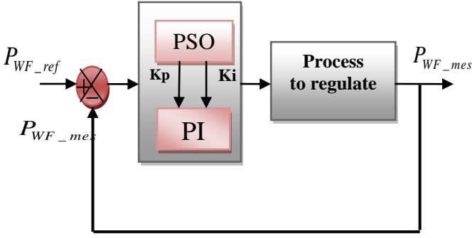
Fig. 5: Block diagram of wind farm supervision system with a PSO-PI controller.
