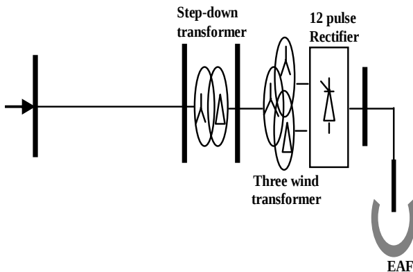
Fig.3 Modelled dc arc furnace plant
