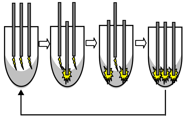
Fig. 9 Cycle of melting proposed
