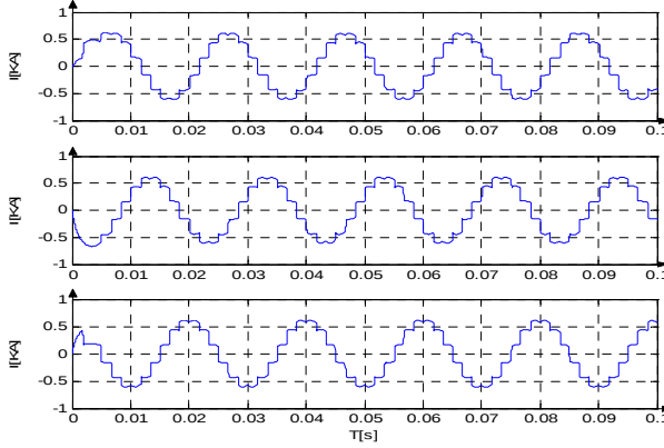
Fig.7 Current of twelve pulse rectifier
