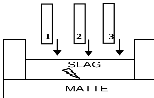
Fig.1 Physical Model of EAF [2]
