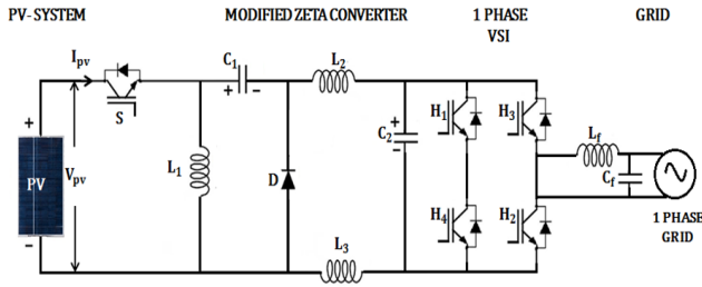
Fig. 2. Proposed System circuit diagram
