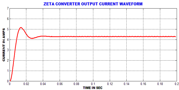
Fig. 11(a). Simulation results of output DC current of the Zeta converter
