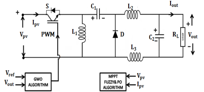
Fig. 1. Proposed high gain DC-DC Zeta Converter
