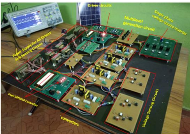
Fig. 5. Hardware Setup
