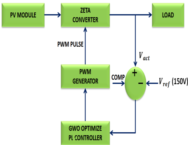
Fig. 3. Control Strategy for Zeta Converter
