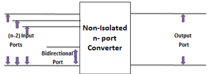
Figure 4 Non-Isolated Multiport DC-DC Converter
