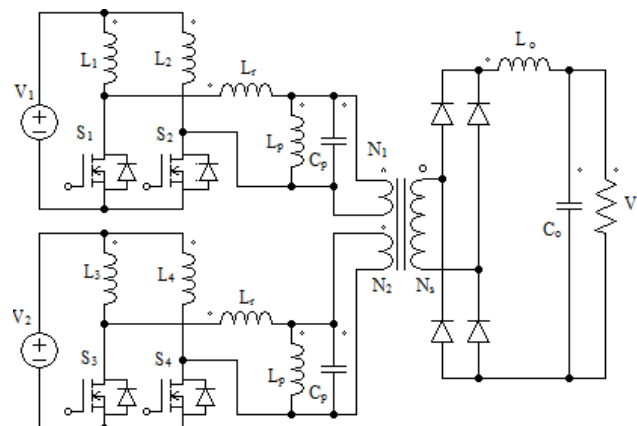
Figure 6 The converter topology in [18]
