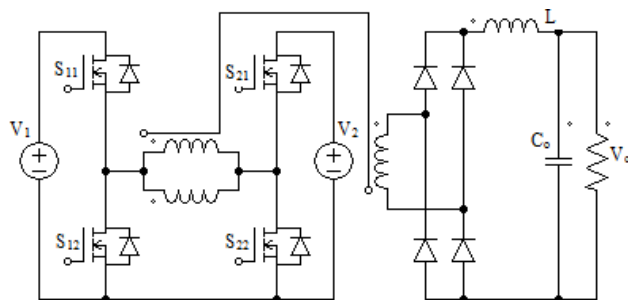
Figure 13 The converter topology in [32]
