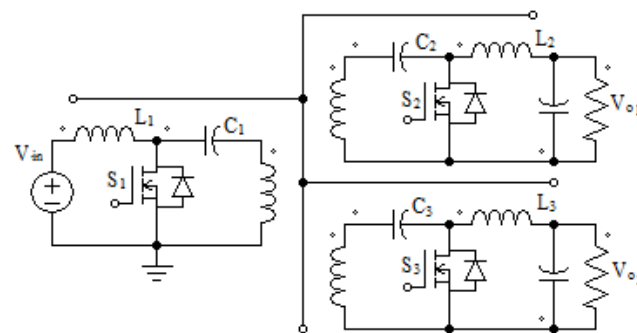
Figure 7 The converter topology in [20]
