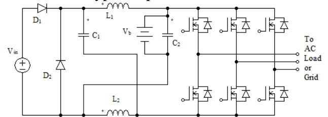
Figure 29 The converter topology in [70]
