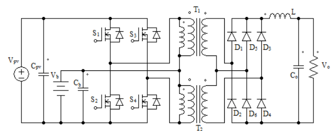
Figure 16 The converter topology in [43]
