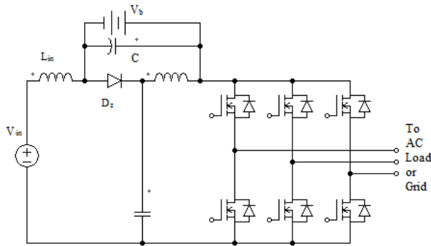
Figure 30 The converter topology in [71]
