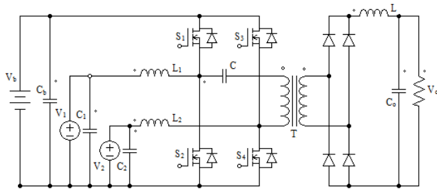
Figure 12 The converter topology in [31]
