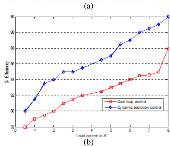
Fig.10. SBC with proposed DE controller (a) Hardware setup (b) Efficiency of two prototype controller
