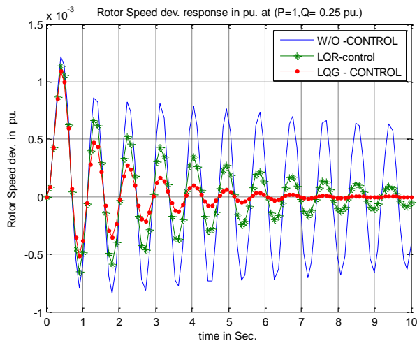
Figure 5 : Rotor speed dev. response due to 0.1 pu load disturbance with and without controllers, at (p=1 pu , Q=.25 pu ).
