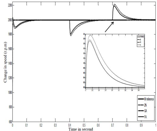
Fig. 7. Change in speed for different algorithms.
