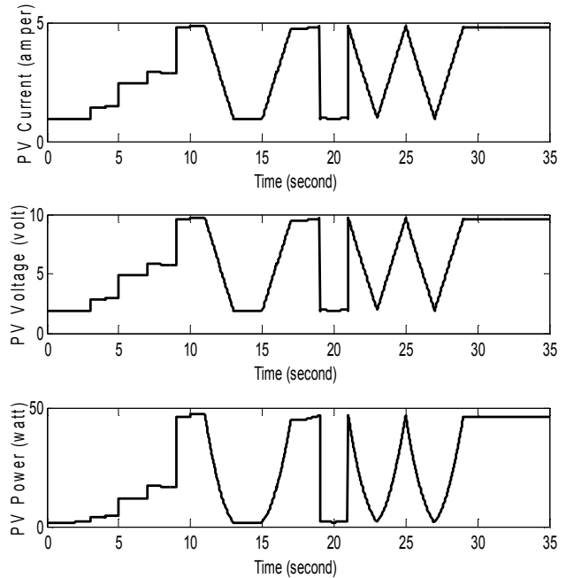
Fig. 15. The PV current, voltage and power.
