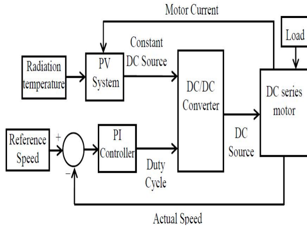
Fig. 1. Block diagram of overall system.
