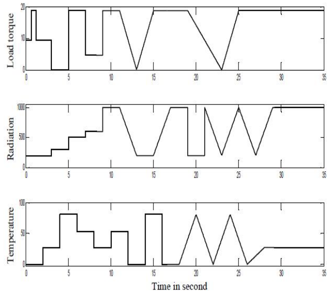
Fig. 14. Change of load torque, PV radiation and temperature.
