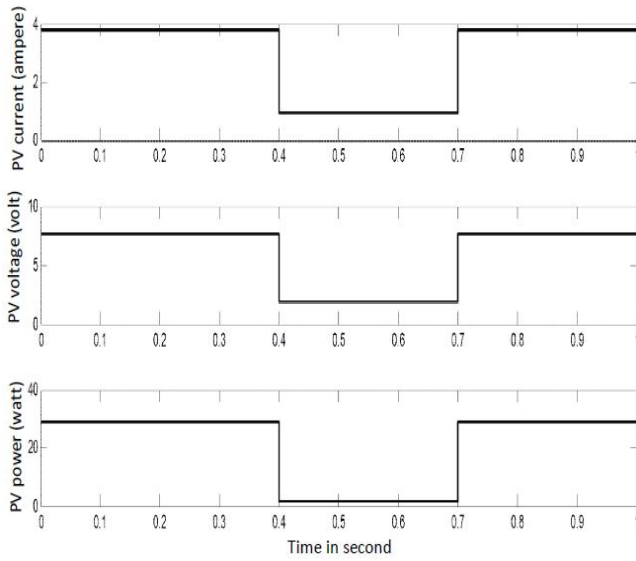
Fig. 12. The PV current, voltage and power.
