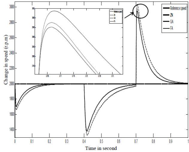
Fig. 10. Change in speed for different controllers.
