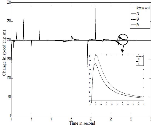
Fig. 16. The change in speed with different controllers.
