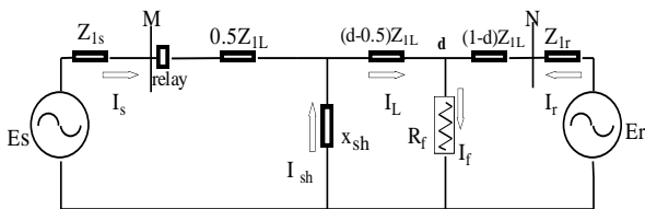
Figure 6. Single line diagram of system for case II.
