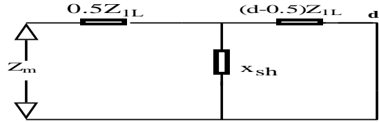
Figure 7. Reduced equivalent circuit during three phase fault at point d.
