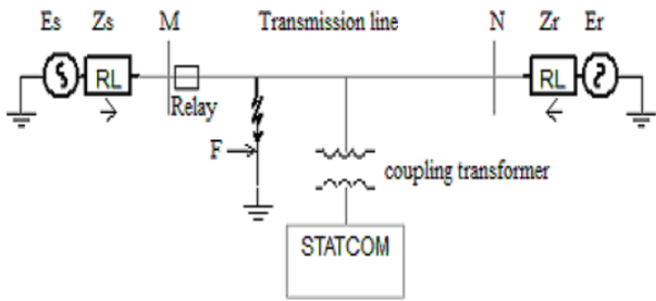
Figure 1. Two generator system with STATCOM.
