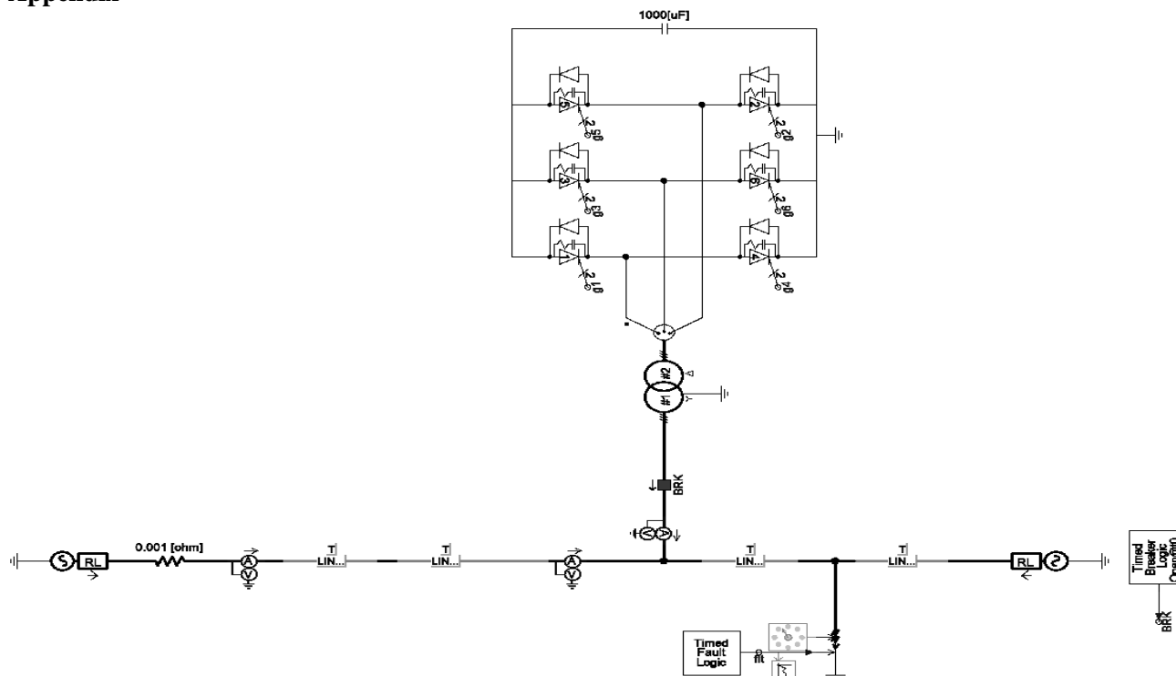
Figure 1. Test system modeled in EMTDC /PSCAD
