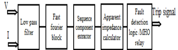
Figure 2. Functional block diagram of the distance relay.
