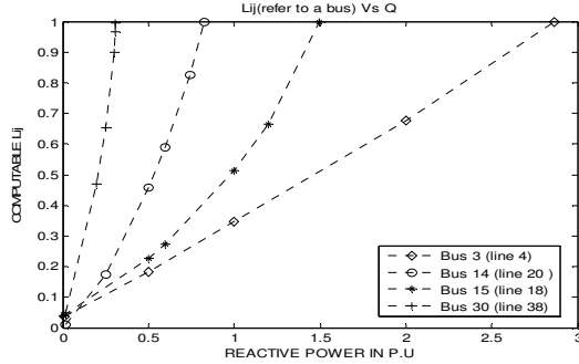
Figure.2. L_{ij} Vs Reactive load variation ( Q )
