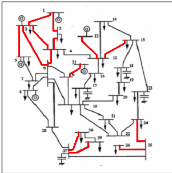
Figure 4. Weak area cluster at Q_3 = 1.432 p.u
