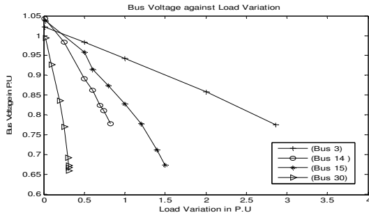
Figure3. Bus voltage against load variation.
